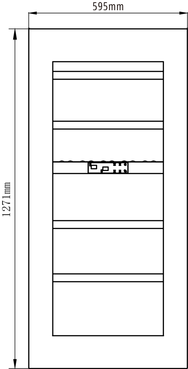
Front View
