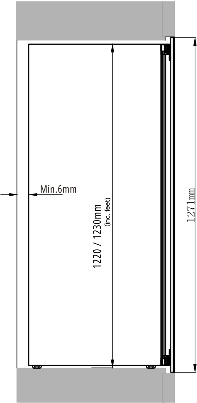
Side View
